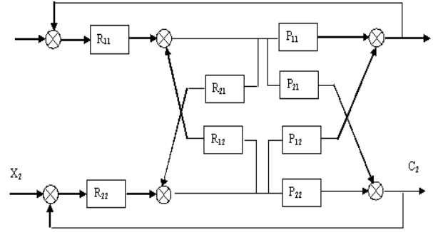
Figure 3. Best decoupling structure of bivariate P normative control object
