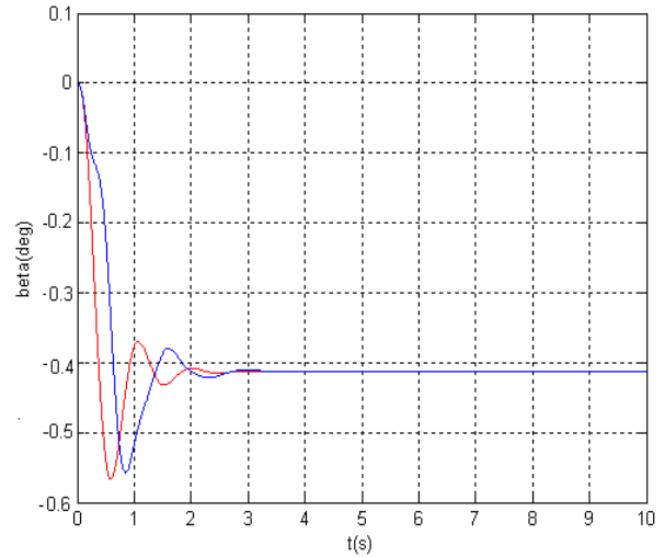
Figure 7. Response curve with Angle of attack
