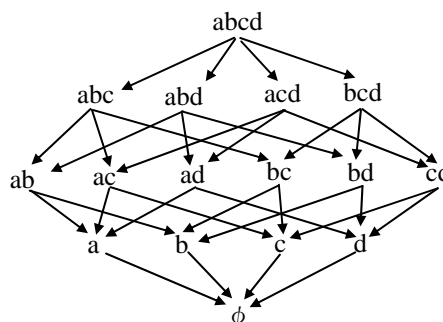
Figure 2. Four dimensional lattice diagram for a data cube
