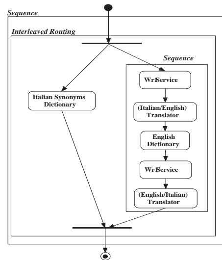
Figure 11. Services Workflow model
