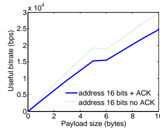
Figure 5. Snapshot of Fig. 4 for an address size of 16 bits. The transition from SIFS to DIFS can be seen clearly
