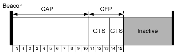
Figure 1. An example of a superframe structure
