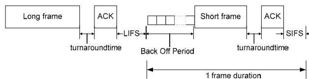
Figure 3. Frame sequence in 802.15.4. We notice the back off period and that long frames are followed by a long inter frame space and short frames by a short inter frame space
