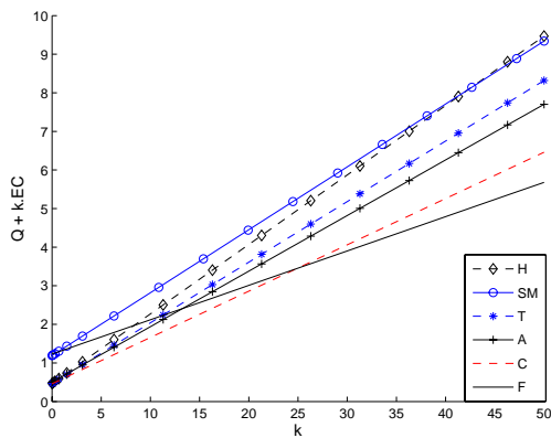
Figure 13. k \rightarrow E(k, R) with internal energy Q for the 6 segmentations R of Fig. 11.
