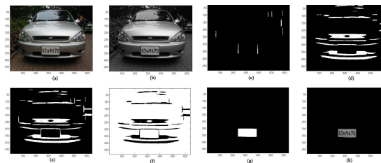
Figure 13. Steps for candidate region detection (white back ground LP).
