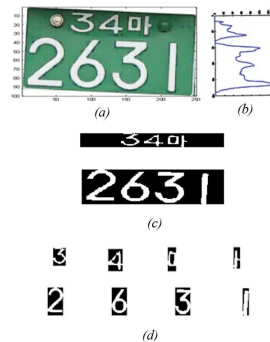
Figure 12. Detect license plate region.
