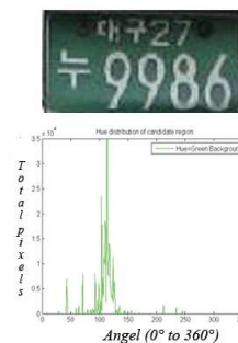
Figure 9. Hue distribution of candidate region.
