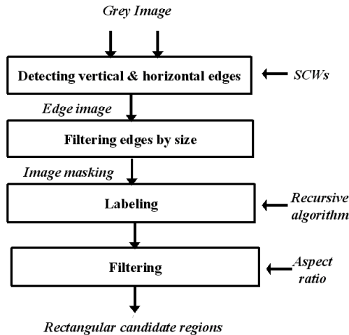
Figure 4. Candidate regions detection.
