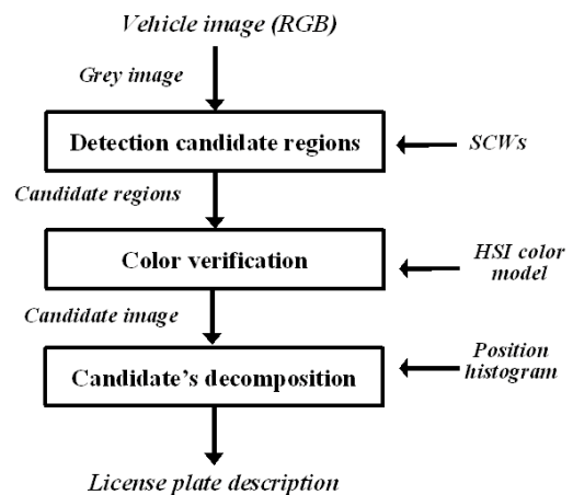
Figure 2. General scheme for detecting license plate region.
