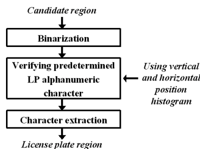
Figure 10. Detect license plate region.
