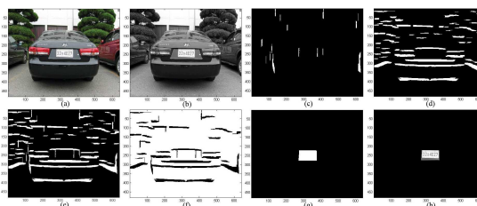
Figure 6. Steps for candidate region detection (white back ground LP).
