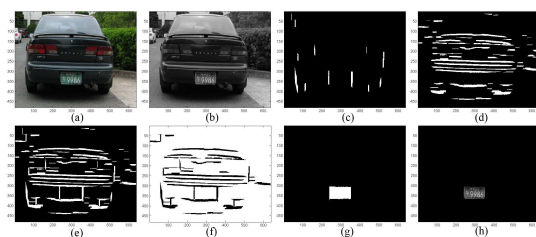
Figure 5. Steps for candidate region detection (green back ground LP).
