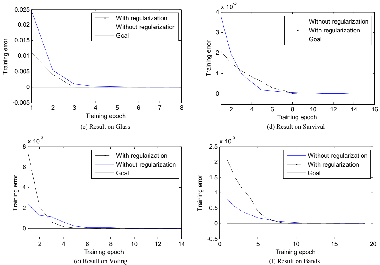
Figure 2. Error curve of SC-RBF network
