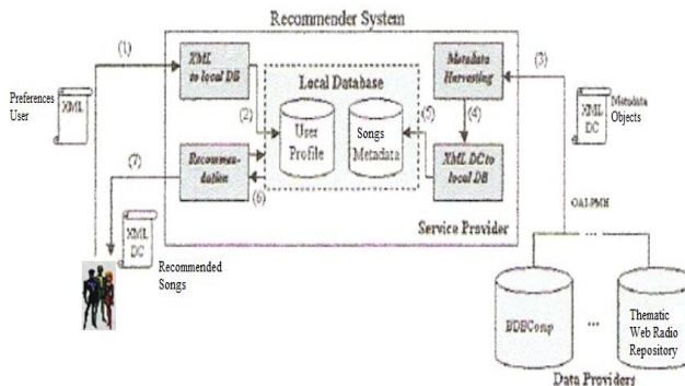
Figure 1. The recommender system architecture.
