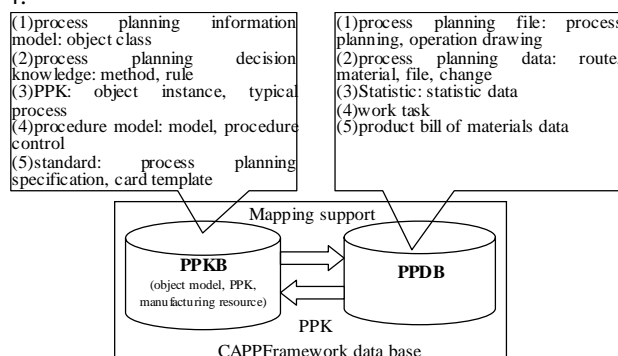
Figure 4. PPDB based on object-oriented information model of PPKB
