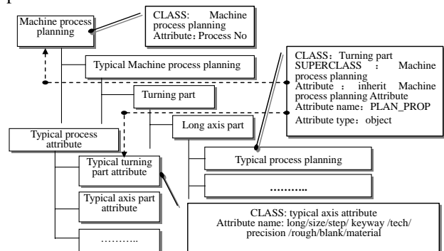
Figure 6. Process planning knowledge model of machining process
