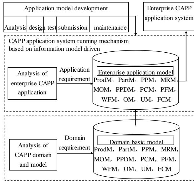
Figure 3. Process planning information model-driven architecture in CAPP database
