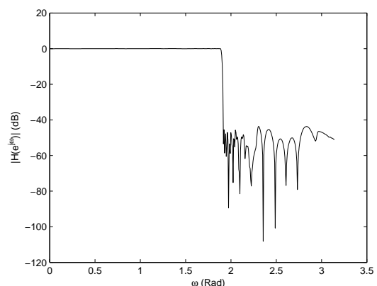
Figure 14. Magnitude Frequency Response of the CSD Lowpass FRM FIR Digital Filter H(z) after GA Optimization
