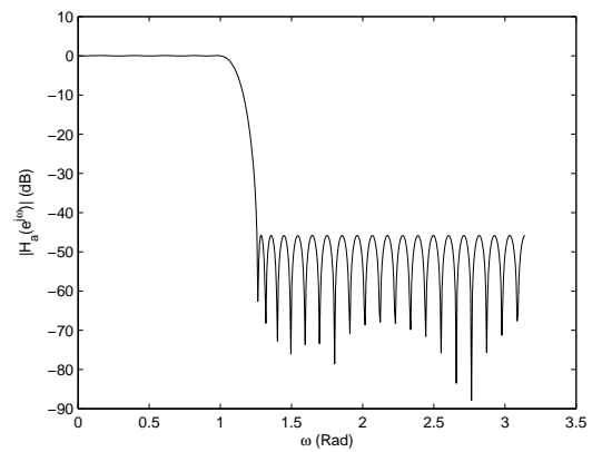
Figure 18. Magnitude Frequency Response of the Digital Subfilter H_a(z)
