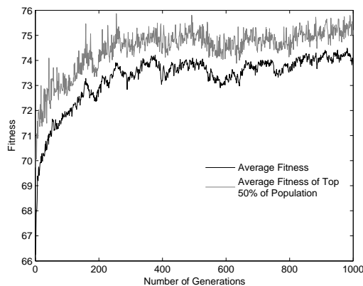
Figure 22. Fitness Evolution for the CSD FRM FIR Bandpass Digital Filter H(z)
