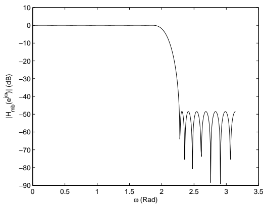
Figure 10. Magnitude Frequency Response of the Masking Digital Subfilter H_{mb}(z)
