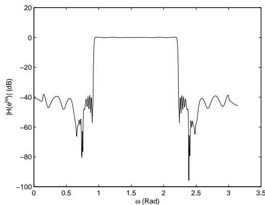
Figure 24. Magnitude Frequency Response of the Bandpass CDBNS FRM Digital Filter H(z) before GA Optimization
