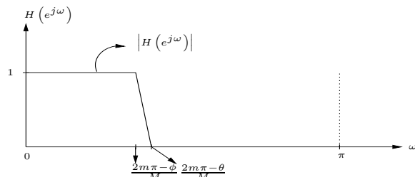
Figure 7. Magnitude Frequency Response of the Overall FRM FIR Digital Filter H(z) [3]
