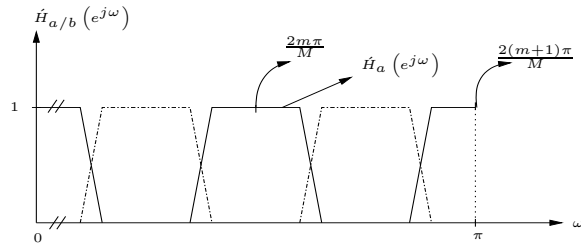
Figure 3. Magnitude Frequency Responses of the M -Interpolated Complementary Digital Subfilters H_a(zM) and H_b(zM) [3]
