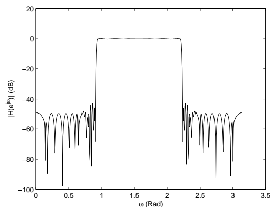
Figure 20. Magnitude Frequency Response of the Infinite-Precision Bandpass FRM FIR Digital Filter H(z)
