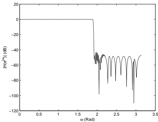
Figure 11. Magnitude Frequency Response of the Infinite-Precision Lowpass FRM FIR Digital Filter H(z)
