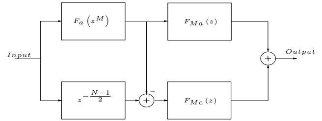
Figure 8. Realization of the Overall FRM FIR Digital Filter H(z)
