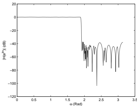
Figure 15. Magnitude Frequency Response of the Lowpass FRM FIR Digital Filter H(z) after CDBNS Approximation
