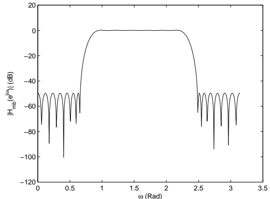
Figure 19. Magnitude Frequency Response of the Masking Digital Subfilter H_{mb}(z)
