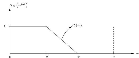
Figure 1. Magnitude Frequency Response of the Bandedge-Shaping Digital Subfilter H_a(z) [3]
