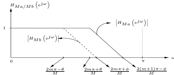
Figure 4. Magnitude Frequency Responses of the Masking Digital Subfilters H_{Ma}(z) and H_{Mb}(z) [3]
