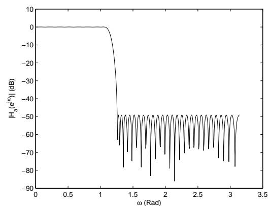
Figure 9. Magnitude Frequency Response of the Digital Subfilter H_a(z)
