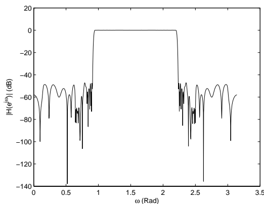
Figure 26. Magnitude Frequency Response of the Bandpass CDBNS FRM Digital Filter H(z) after GA Optimization
