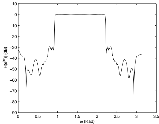
Figure 21. Magnitude Frequency Response of the Bandpass FRM FIR Digital Filter H(z) after CSD Approximation
