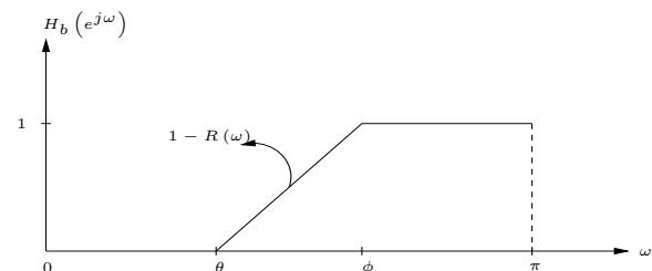
Figure 2. Magnitude Frequency Response of the Complementary Bandedge-Shaping Digital Subfilter H_b(z) [3]
