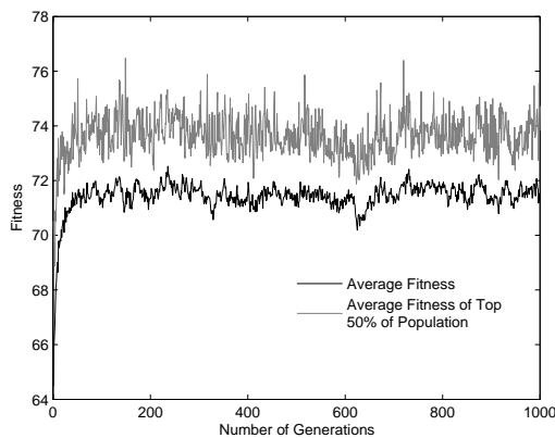
Figure 25. Fitness Evolution for CDBNS FRM FIR Bandpass Digital Filter
