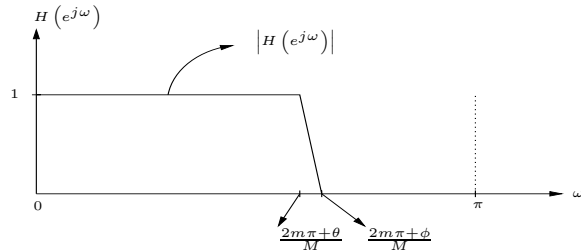
Figure 5. Magnitude Frequency Response of the Overall FRM FIR Digital Filter H(z) [3]
