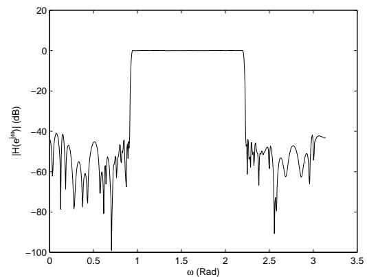
Figure 23. CSD Bandpass FRM FIR Digital Filter H(z) after GA Optimization
