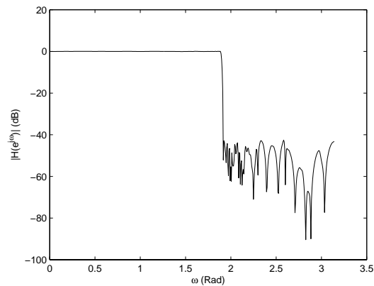
Figure 17. Magnitude Frequency Response of the CDBNS Lowpass FRM FIR Digital Filter H_{LP}(z) after GA Optimization
