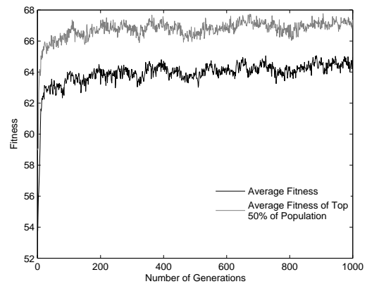
Figure 13. Fitness Evolution for CSD FRM FIR Lowpass Digital Filter H(z)
