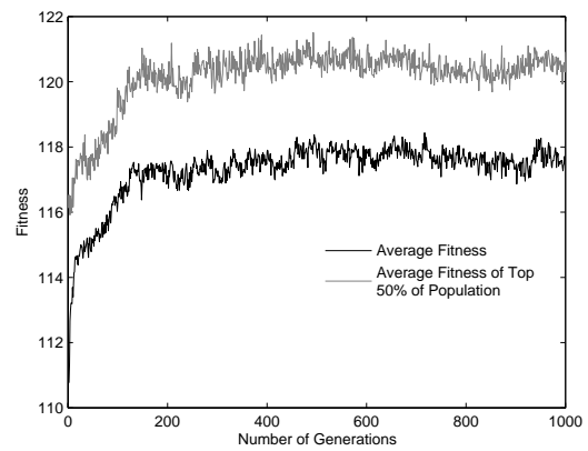
Figure 16. Fitness Evolution for the CDBNS Lowpass FRM FIR Digital Filter H(z)
