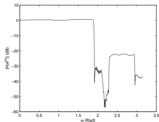
Figure 12. Magnitude Frequency Response of the Lowpass FRM FIR Digital Filter H(z) after CSD Approximation
