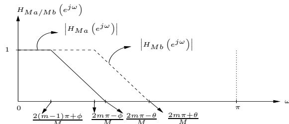
Figure 6. Magnitude Frequency Response of the Masking Digital Subfilters H_{Ma}(z) and H_{Mb}(z) [3]
