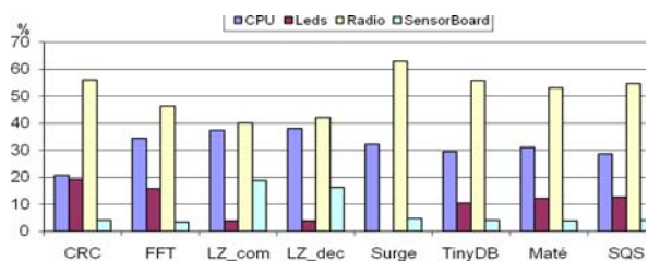
Fig. 11. Energy dissipation of components in MICA2 platform
