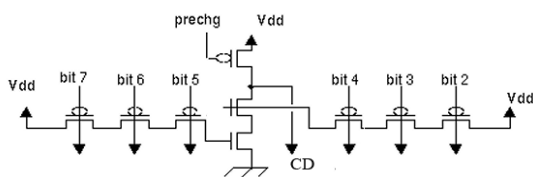
Fig. 6. Encoding logic for the Common Data (CD) bit
