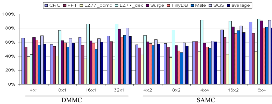
Fig. 8. Average savings on memory access energy dissipation for various MC configurations with the silent-store filter (s x a, s: set no, a: associativity)
