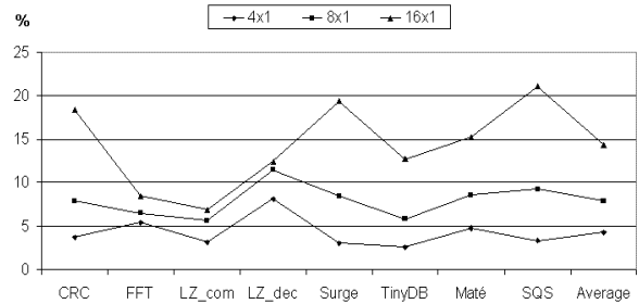
Fig. 13. Possible performance improvements in DMMC configurations
