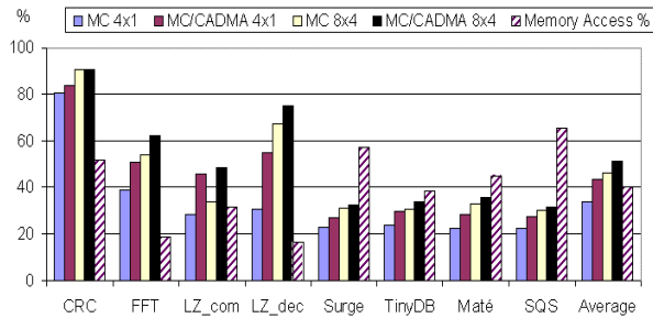
Fig. 10. Processor energy savings and percentages of memory access
