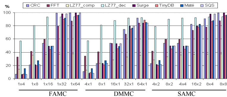
Fig. 3. Hit ratios to various MC configurations (s x a, s: set no, a: associativity)
