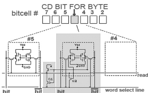
Fig. 7. The CD bit and associated logic common to six most significant bitcells within byte
