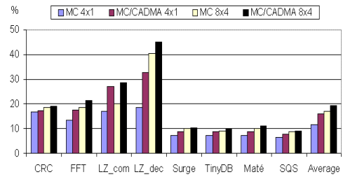
Fig. 12. Node-level energy savings and lifetime improvements
