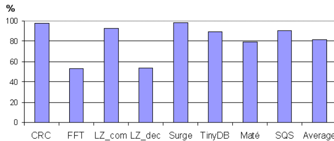
Fig.4. Percentages of silent stores in WSN benchmarks
