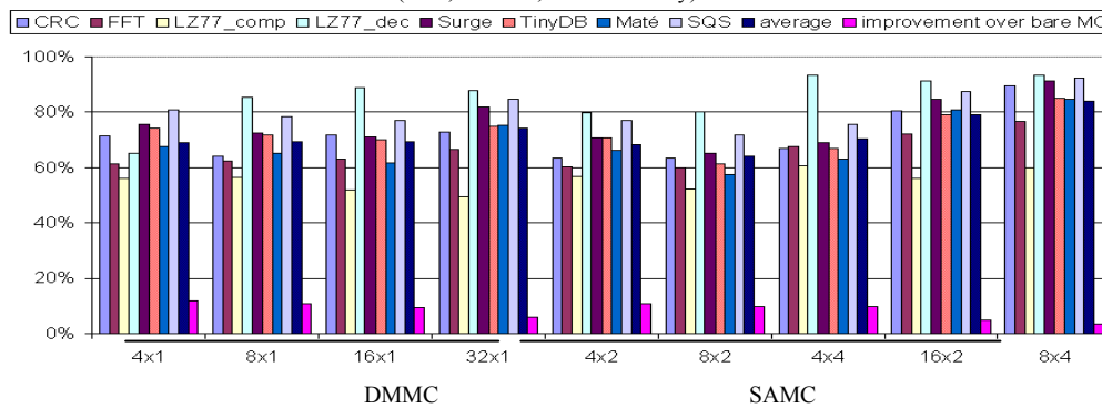
Fig. 9. Average savings on memory access energy dissipation for MC/CADMA
