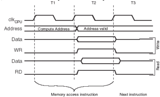
Fig. 1. On-chip Data SRAM access cycles for ATmega128L.
