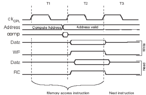
Fig. 2. Modified On-chip Data SRAM and MC access cycles
