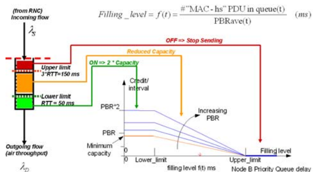
Fig. 4: Flow control mechanism and credit calculation
