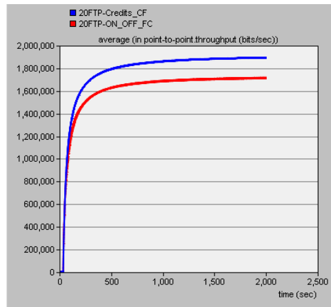
Fig. 8: Average ATM link throughput
