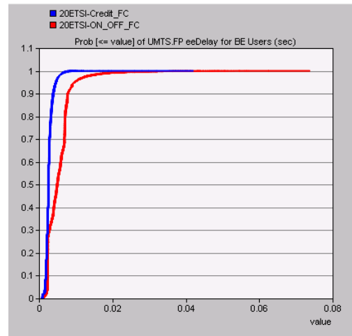
Fig. 18: Average FP end-to-end delay
