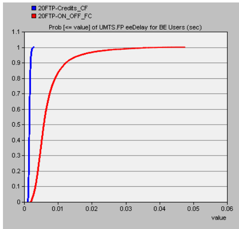
Fig. 10: CDF of FP end-to-end delay
