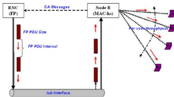
Fig. 5: Functional description of flow control in HSDPA
