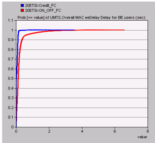
Fig. 20: The CDF of MAC-d end-to-end delay
