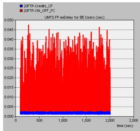
Fig. 9: FP end-to-end delay
