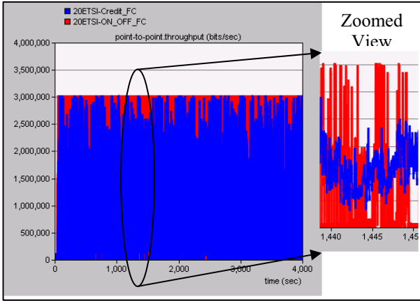
Fig. 14: ATM link throughput
