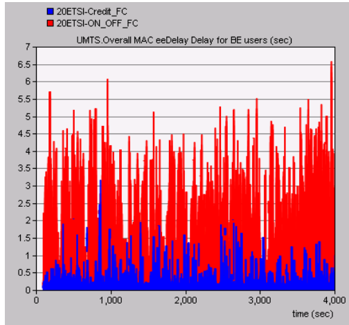
Fig. 19: MAC-d end-to-end delay
