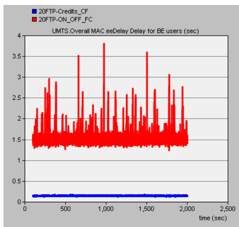
Fig. 11: MAC-d end-to-end delay
