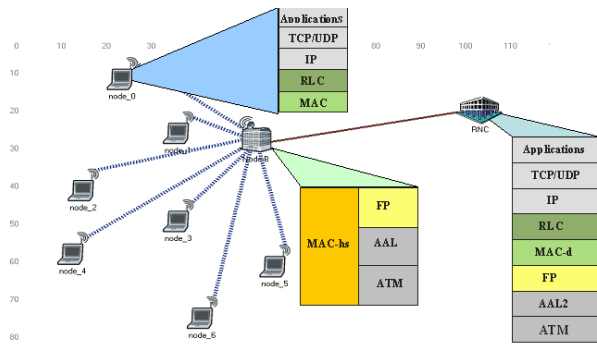
Fig. 1: Simplified UTRAN Architecture (HSDPA)
