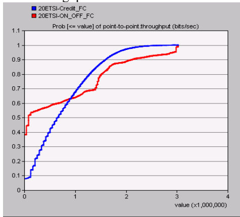
Fig. 15: CDF of ATM link throughput
