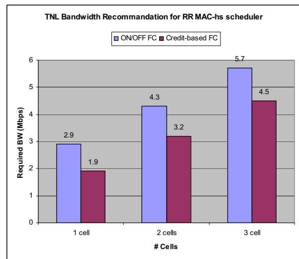
Fig. 22: TNL BW recommendation for RR MAC-hs scheduler based configuration
