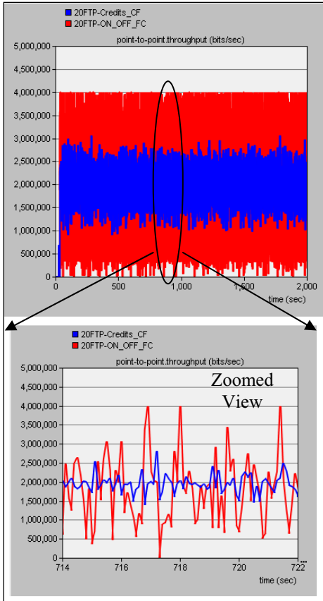
Fig. 6: ATM link throughput
