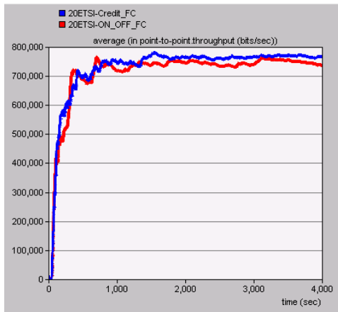
Fig. 16: Average ATM link throughput
