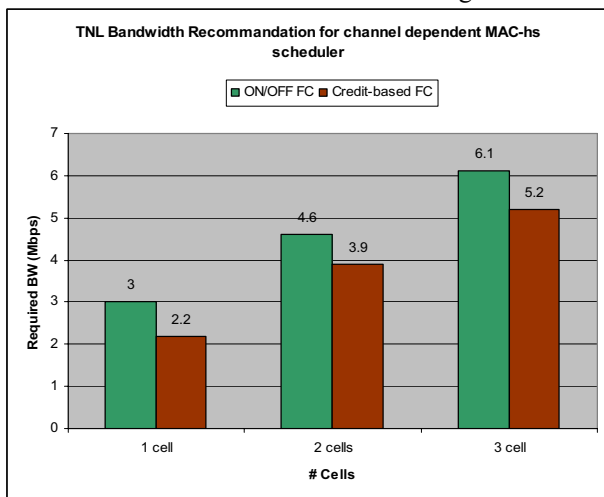
Fig. 23: TNL BW recommendation for channel dependent MAC-hs scheduler based configuration
