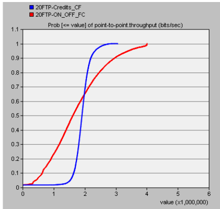
Fig. 7: CDF of ATM link throughput
