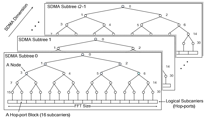
Fig. 8. SDMA channel resource trees (FFT size=256 as shown).
