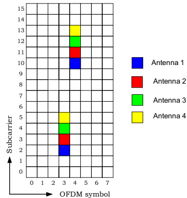
Fig. 13. BRCH mode common pilot placement.
