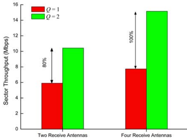
Fig. 9. Forward link sector throughput/5 MHz ( M_T = 4 , M_R = 2 and 4 , 3km/h Pedestrian B channel, 16 access terminals per sector).
