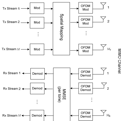
Fig. 1. MIMO spatial multiplexing diagram.
