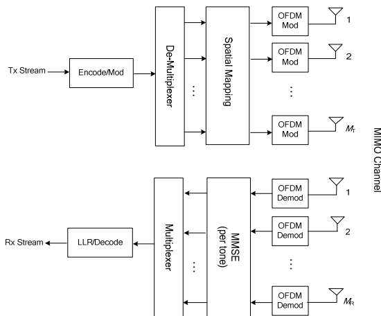
Fig. 3. Illustration of single code word MIMO.
