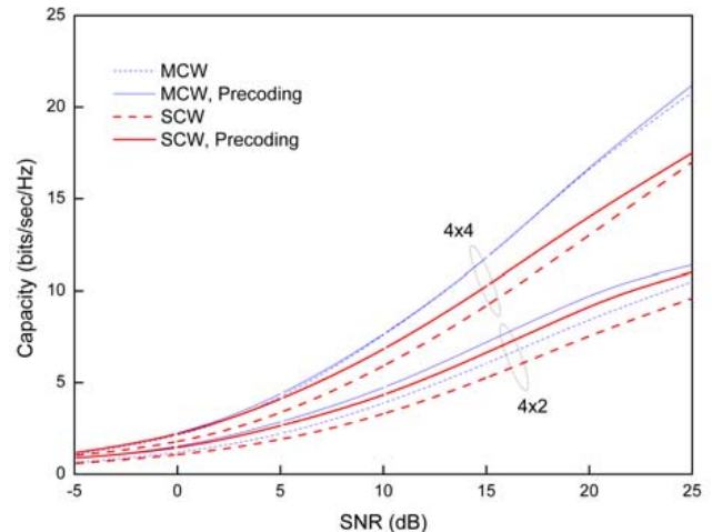
Fig. 6. Precoding gain (64 QAM constellation, PedB channel model).
