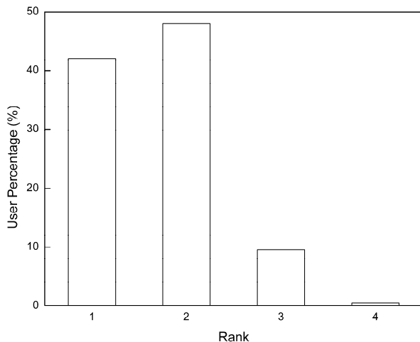
Fig. 4. Rank distribution in a 4 \times 4 MIMO system.
