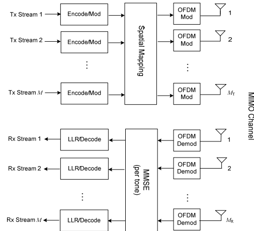
Fig. 2. Illustration of multiple codeword MIMO.
