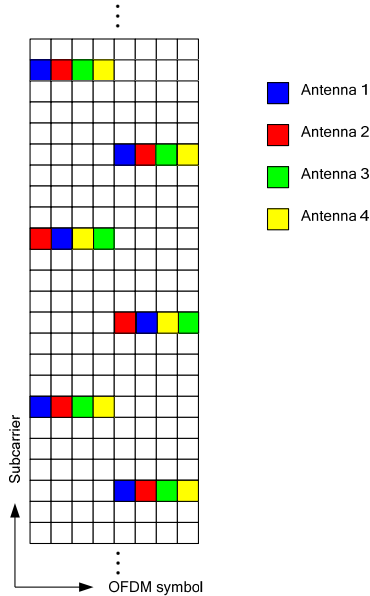
Fig. 11. Illustration of forward common pilot placement ( M_T = 4 ).
