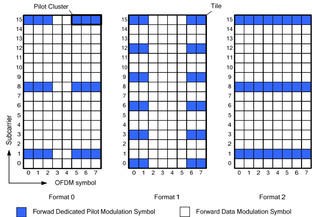
Fig. 12. Illustration of forward dedicated pilot placement within a tile where M_c = 3, 2, and 8 for Formats 0, 1, and 2, respectively.
