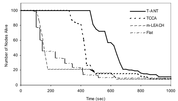
Figure 5. Network lifetime against simulation time of T-ANT, TCCA, m-LEACH and the flat strategy.
