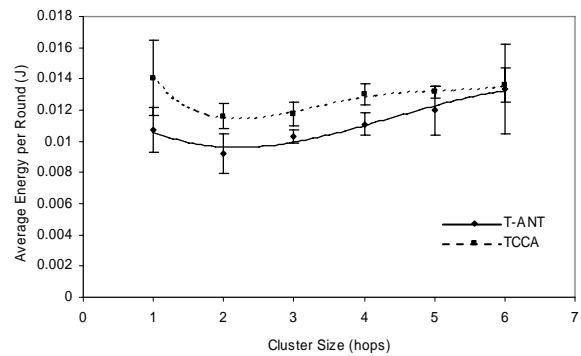
Figure 4. Average energy usage per round against the cluster size of T-ANT and TCCA (and m-LEACH similar to TCCA with cluster size one).
