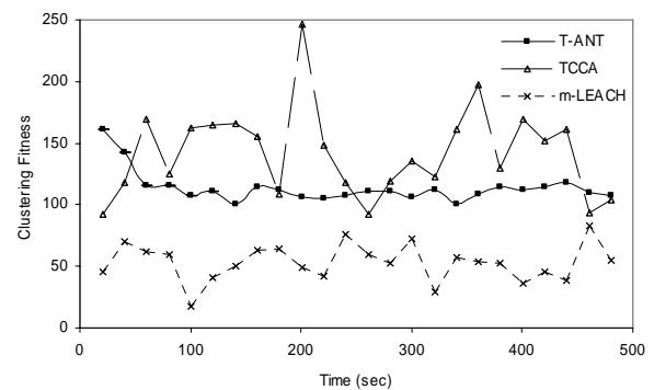
Figure 2. Clustering fitness at different simulation time of T-ANT, m-LEACH and TCCA.
