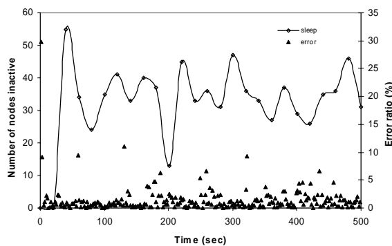
Figure 7. Number of inactive nodes (i.e. sleeping) shown on the primary y-axis against simulation time. The secondary y-axis shows the error ratio between the two values.
