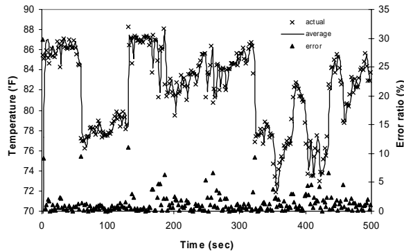
Figure 6. Actual and predicted temperature data values of a single node shown on the primary y-axis against simulation time. The secondary y-axis shows the error ratio between the two values.
