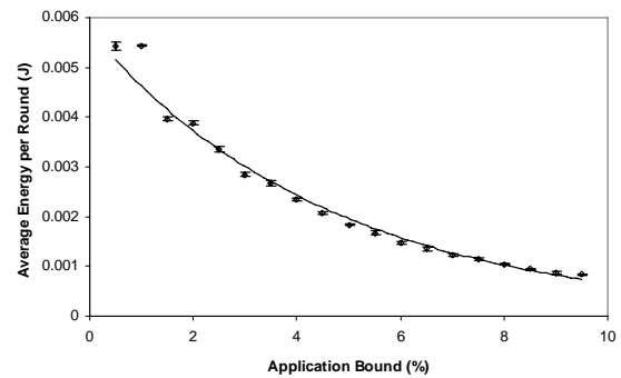
Figure 8. Average energy cost per data collection round against the application bound.
