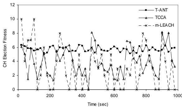
Figure 3. CH election fitness at different simulation time of T-ANT, m-LEACH and TCCA.
