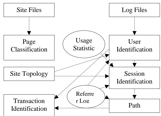
Figure 1. Web Usage Mining Process
