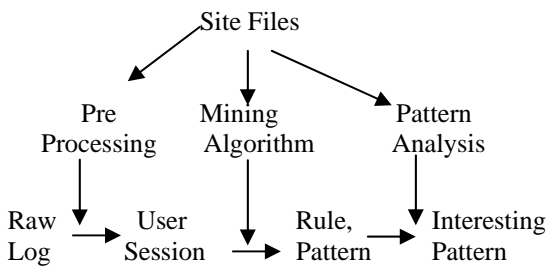
Figure 2. Generalized Web Mining
